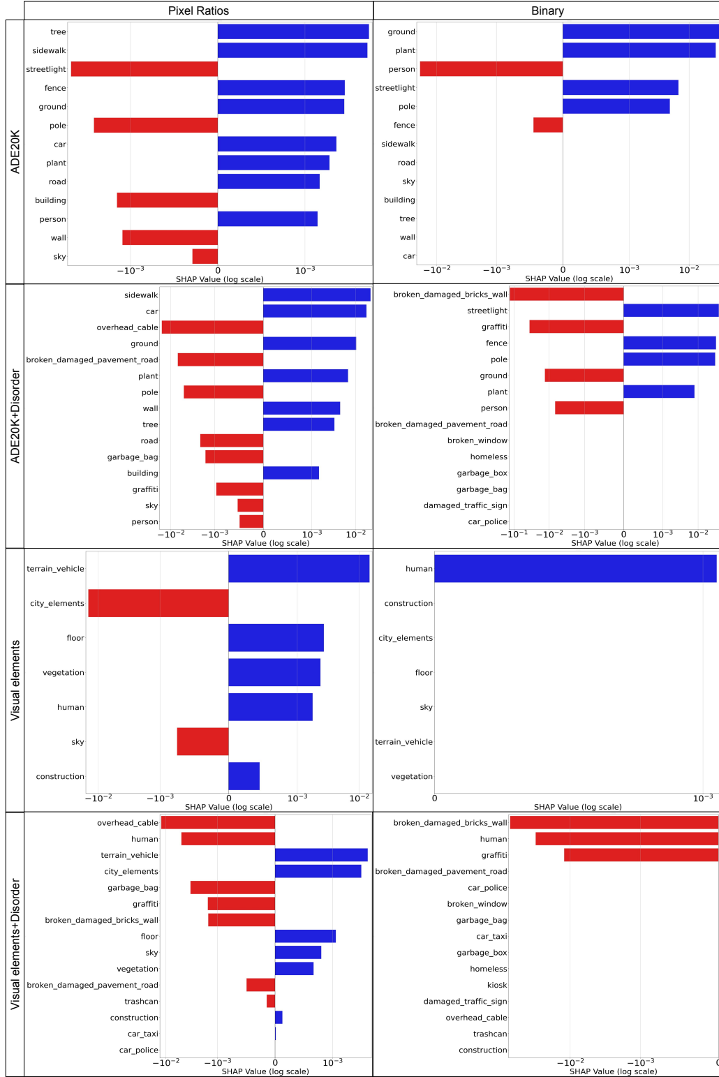
Fig. 3. SHAP values for both: binary presence and pixel ratios values.
