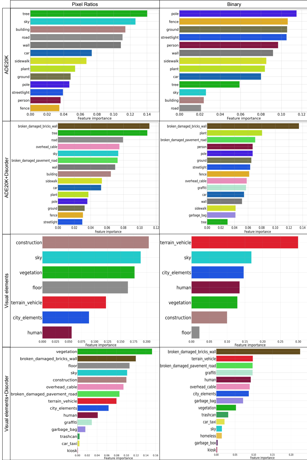
Fig. 2. Feature importance of the top 15 elements in all models evaluated.
