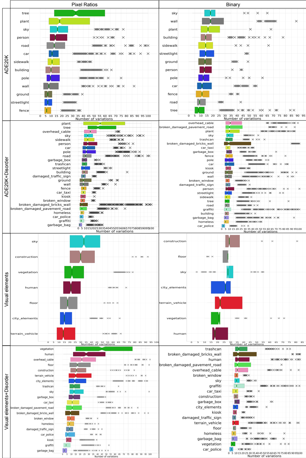
Fig. 4. Measure influence of elements by generating 100 Counterfactuals generations.
